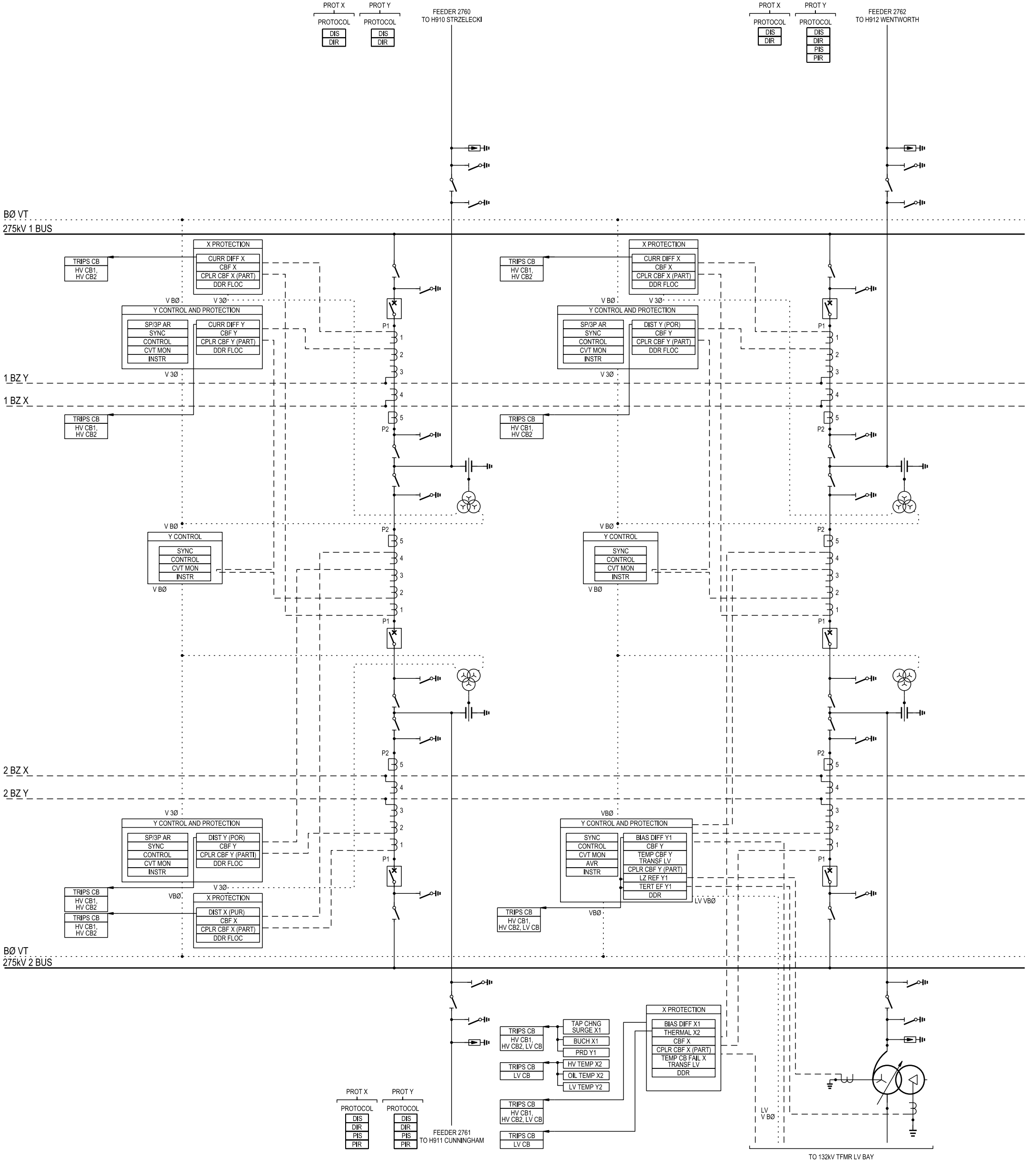
TYPICAL 275kV SECONDARY SYSTEMS LINE DIAGRAM
