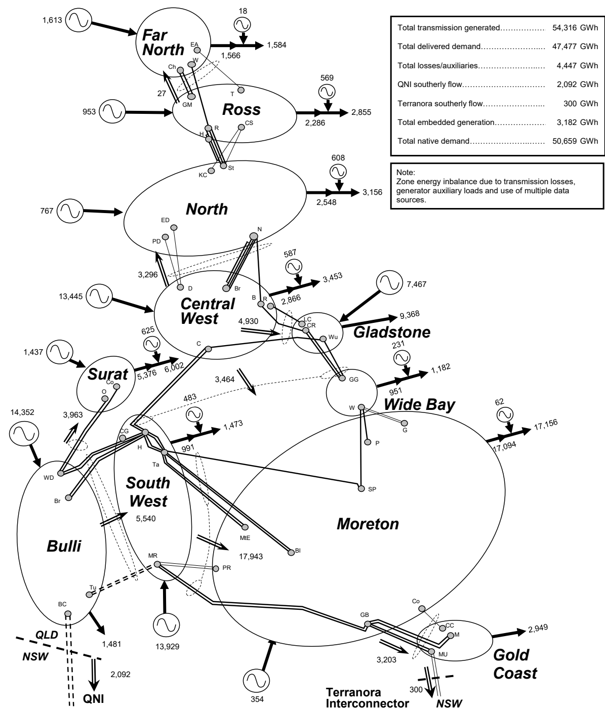
Figure 7.8 2023/24 zonal electrical energy transfers (GWh)
