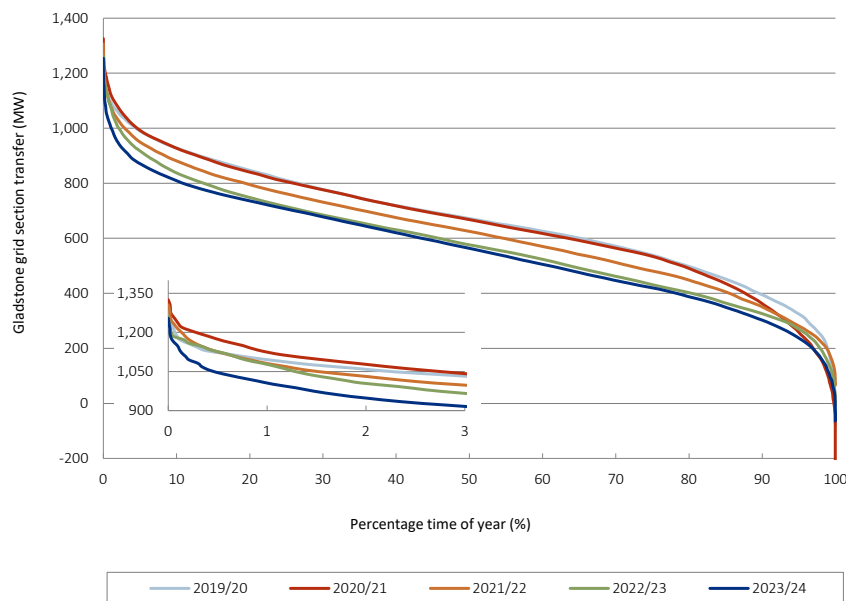
Figure 7.17 Historical Gladstone grid section transfer duration curves
