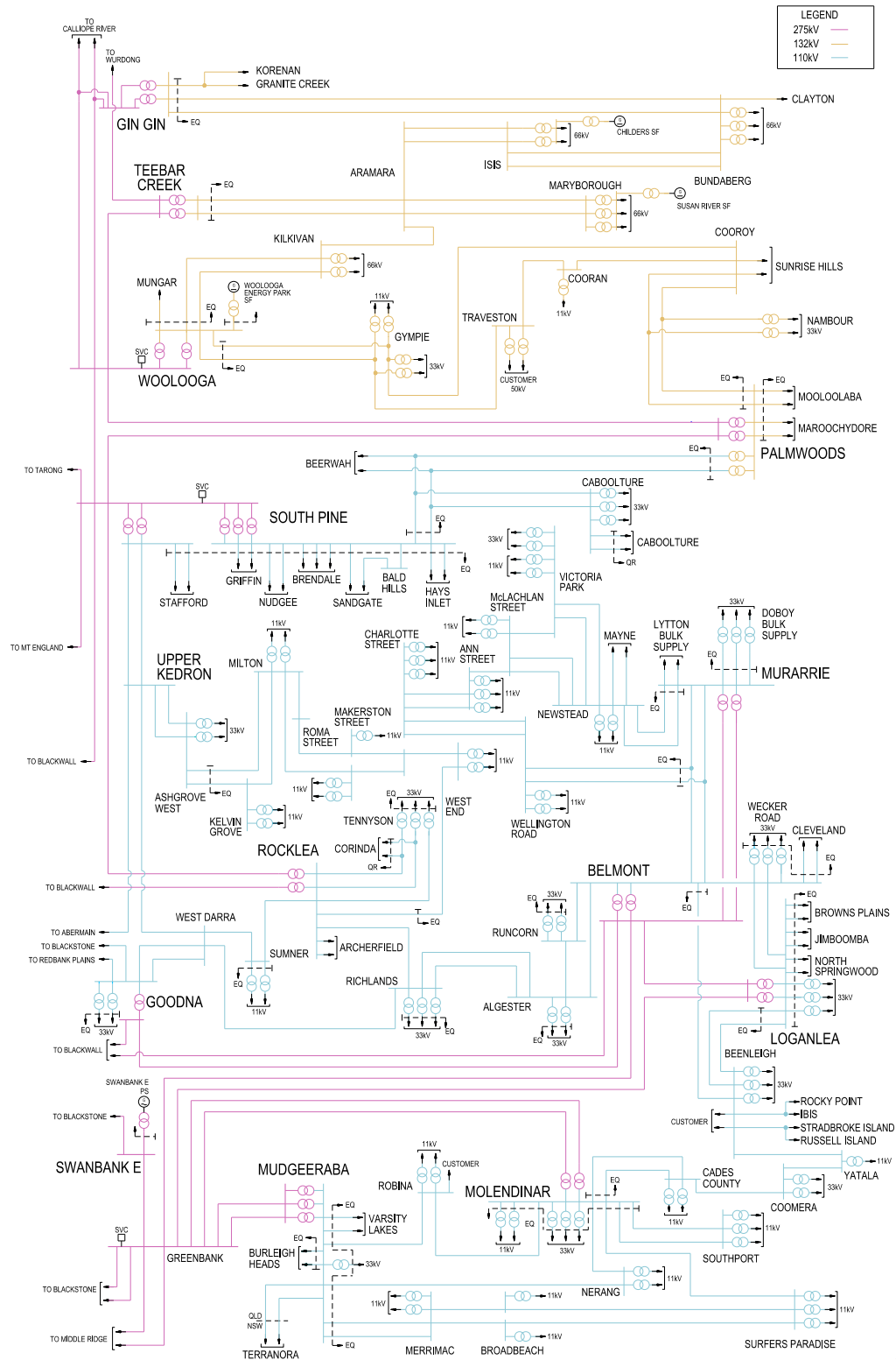
Figure 7.6 Existing HV network July 2024 - South East Queensland
