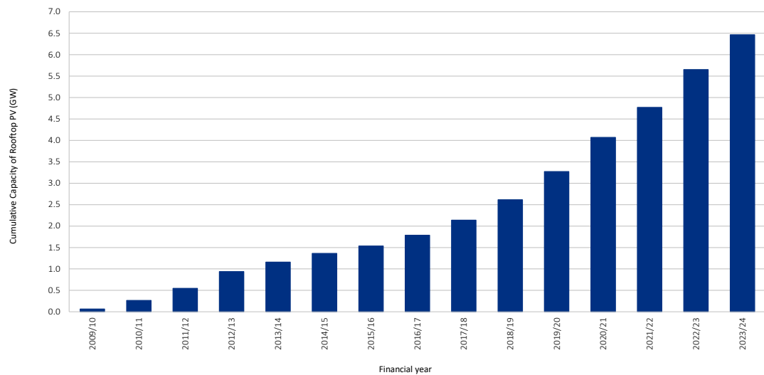
Figure 3.5 Cumulative capacity of Queensland rooftop PV (1) (2)
