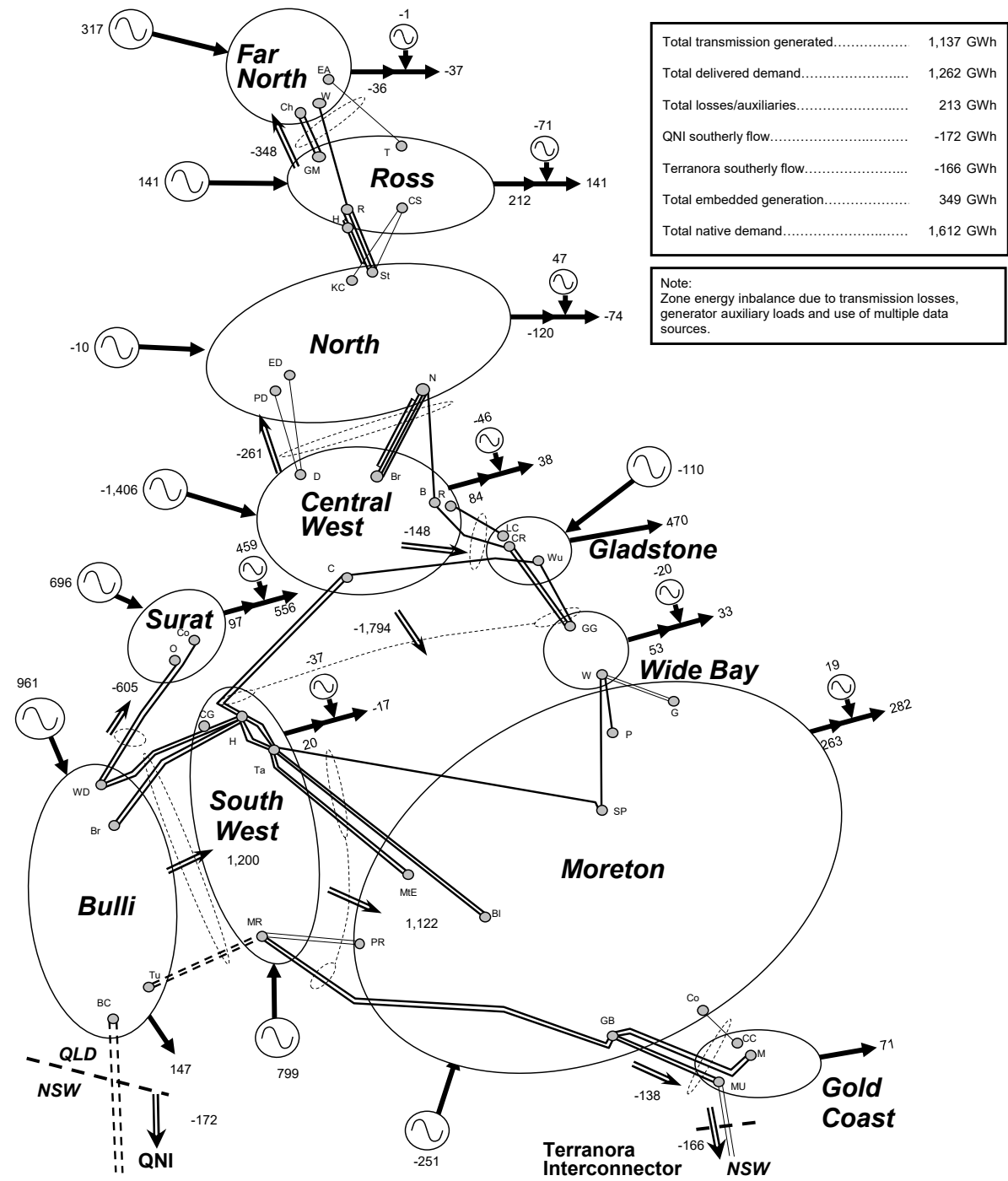
Figure 7.9 Change in zonal electrical energy transfers (GWh)
