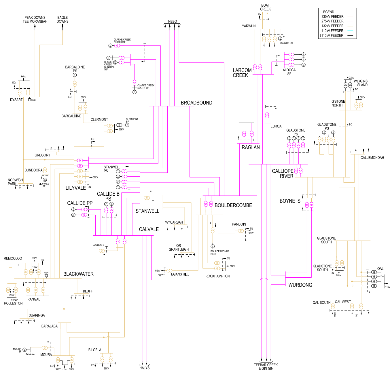
Figure 6.4 Existing HV network, July 2025 – Central Queensland
