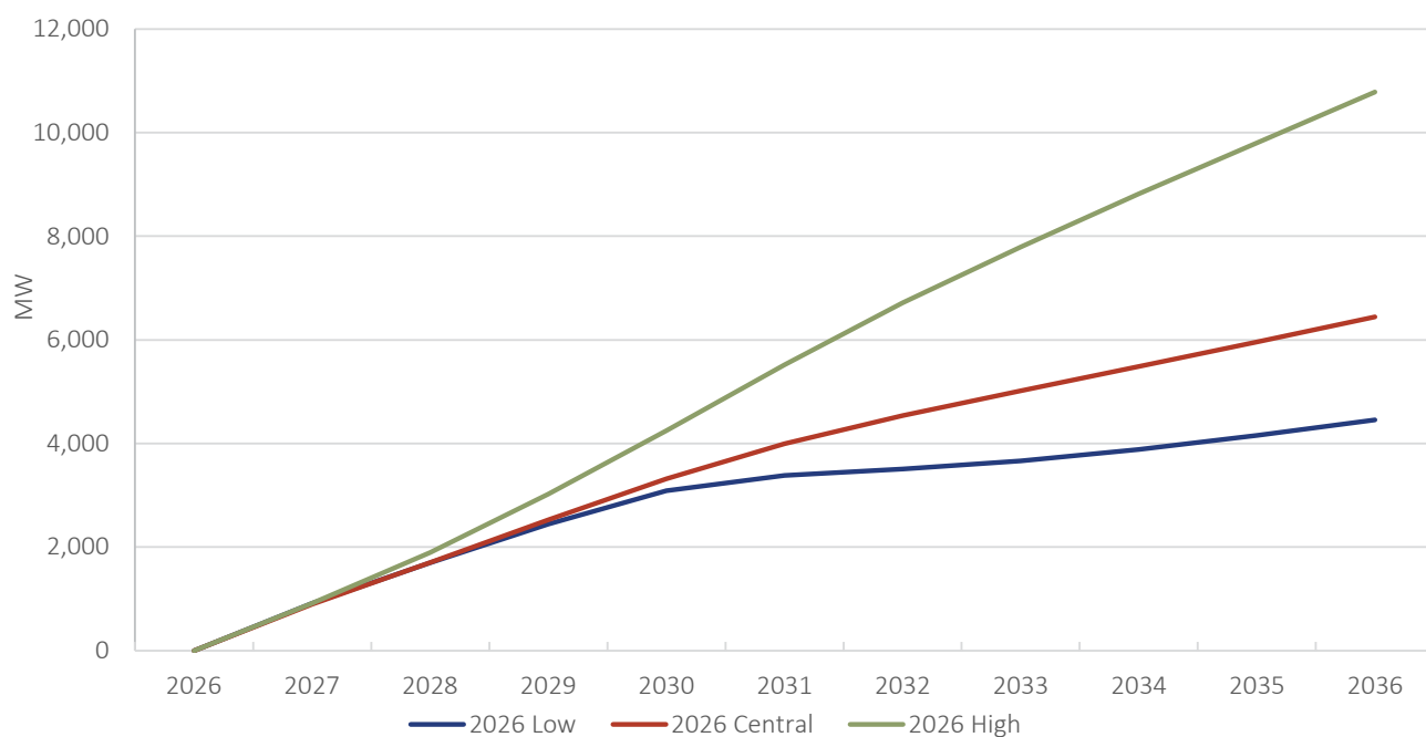
Figure E.4 Embedded Battery Energy Storage System – Capacity
