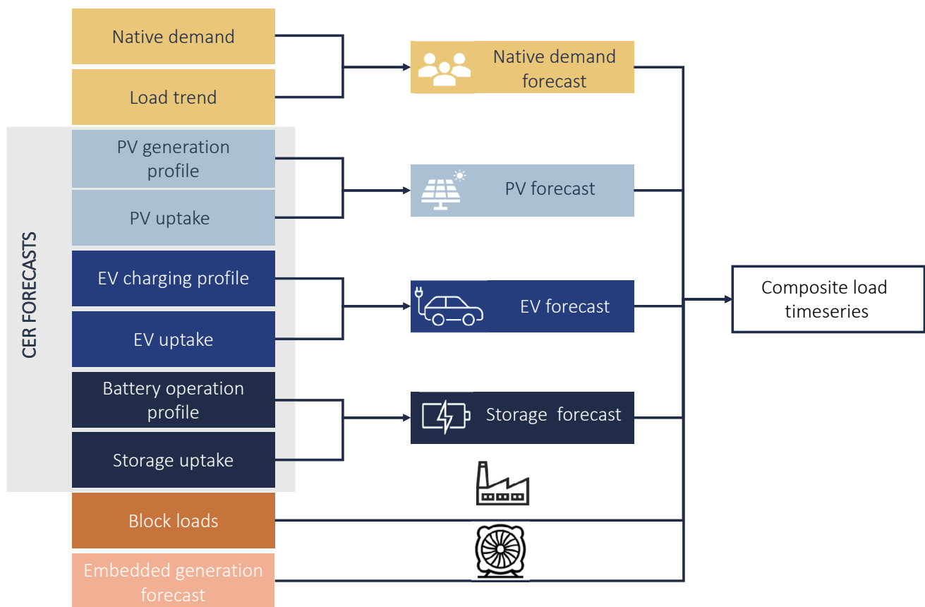
Figure E.1 Schematic of the building blocks of the forecast
