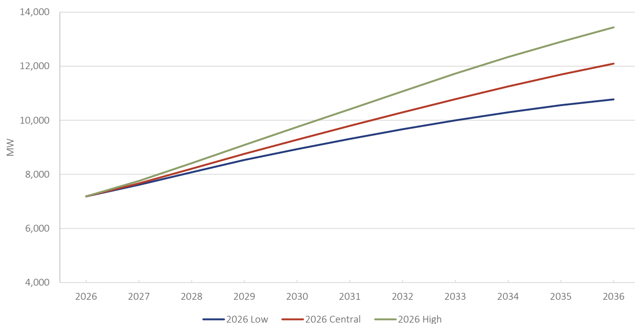
Figure E.6 Rooftop PV uptake – Capacity
