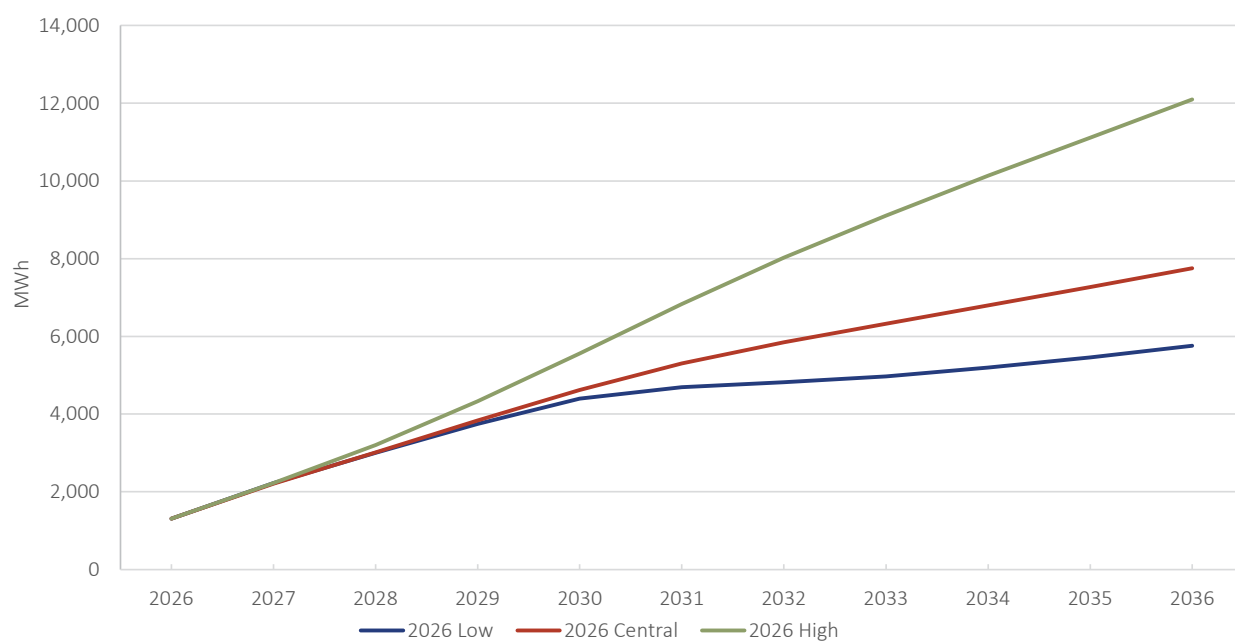
Figure E.5 Embedded Battery Energy Storage System – Energy
