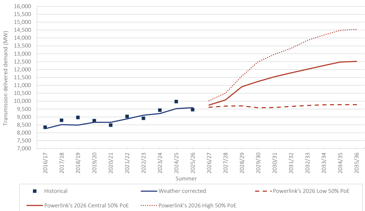
Figure 2.15 Historical and forecast transmission-delivered summer maximum demand
