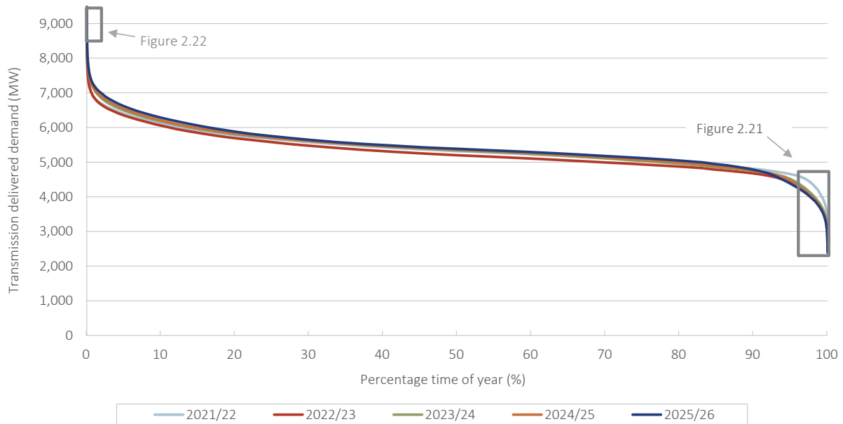
Figure 2.20 Historical transmission-delivered load duration curve
