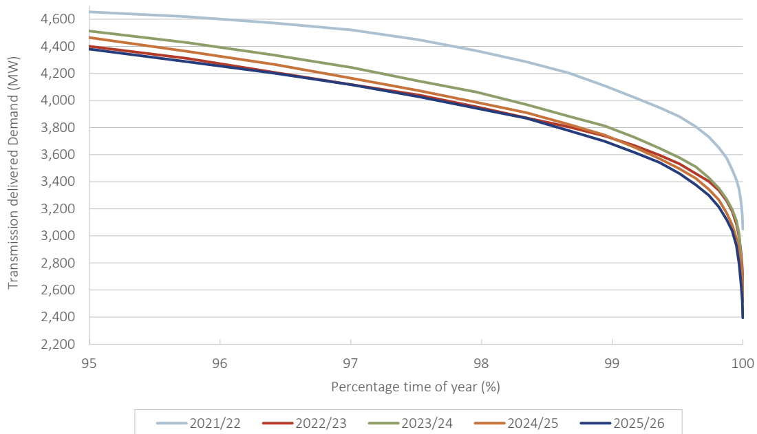
Figure 2.21 Historical transmission-delivered load duration curves (95-100%)
