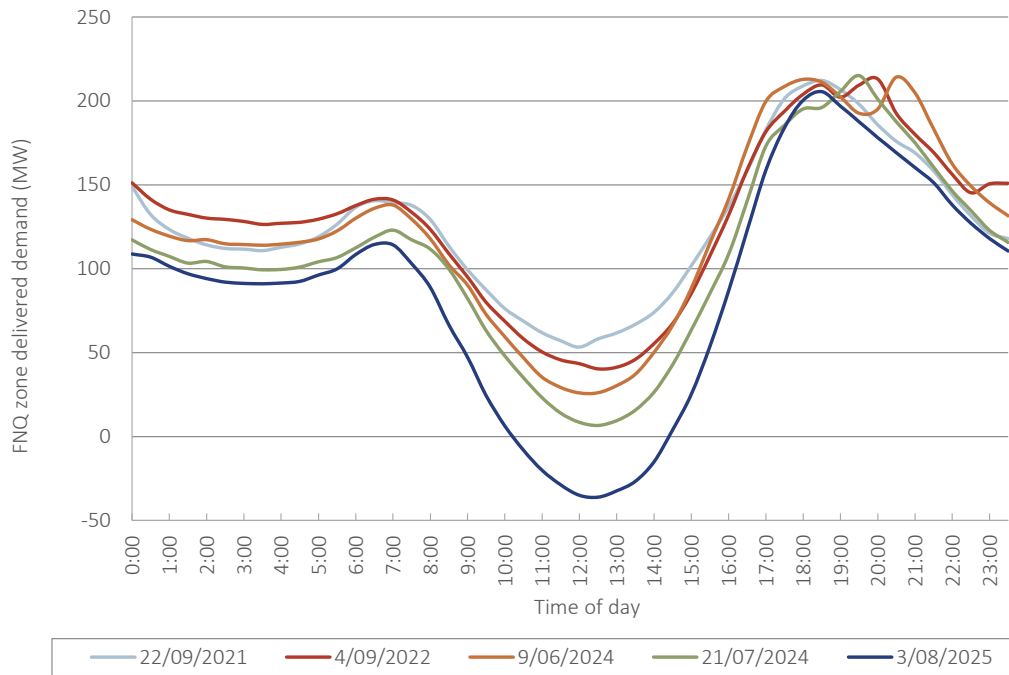
Figure 9.6 Far North daily profile of minimum demand days over the last five years
