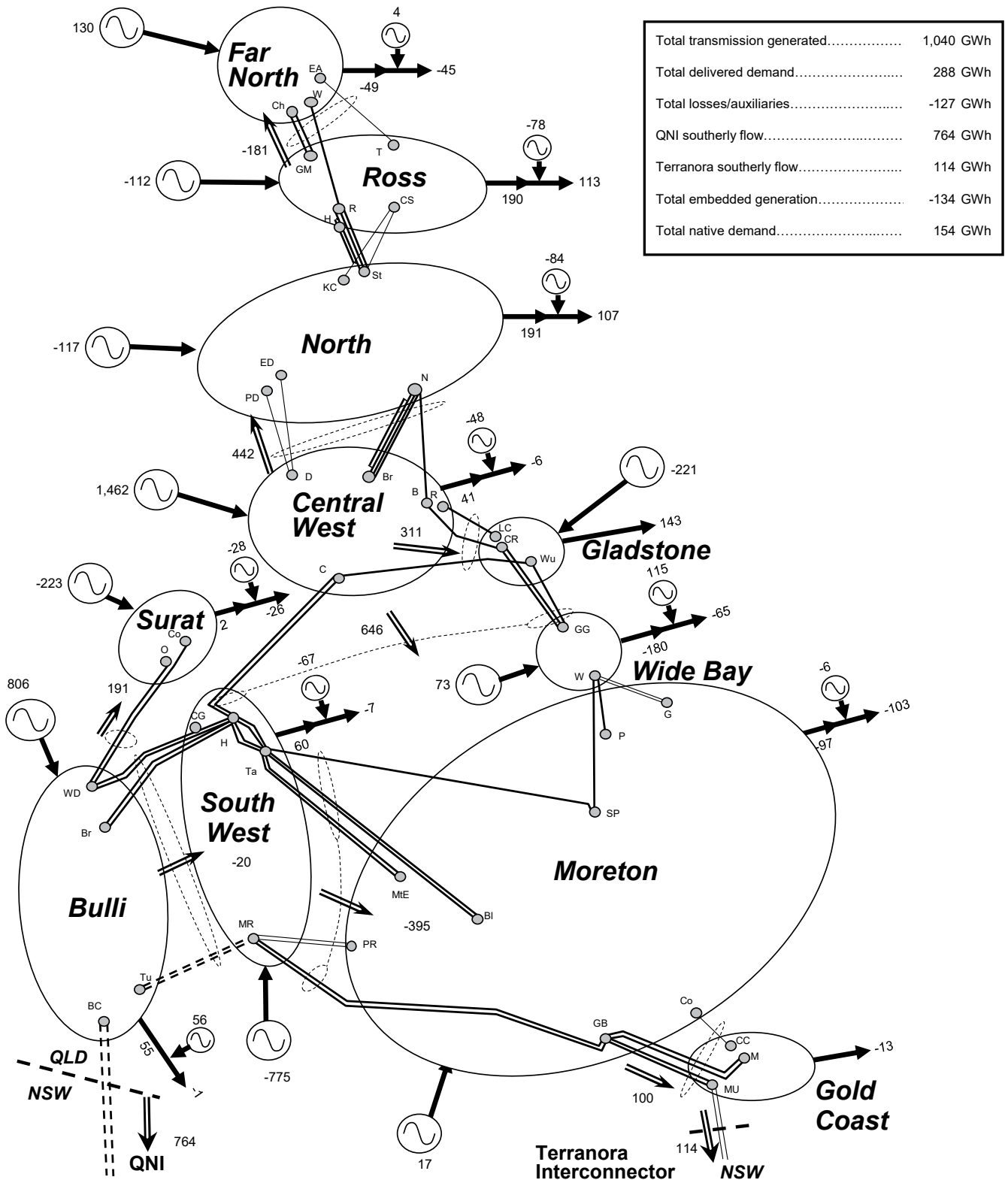
Figure 9.5 Change in zonal electricity transfers (GWh), 2024/25 to 2025/26
