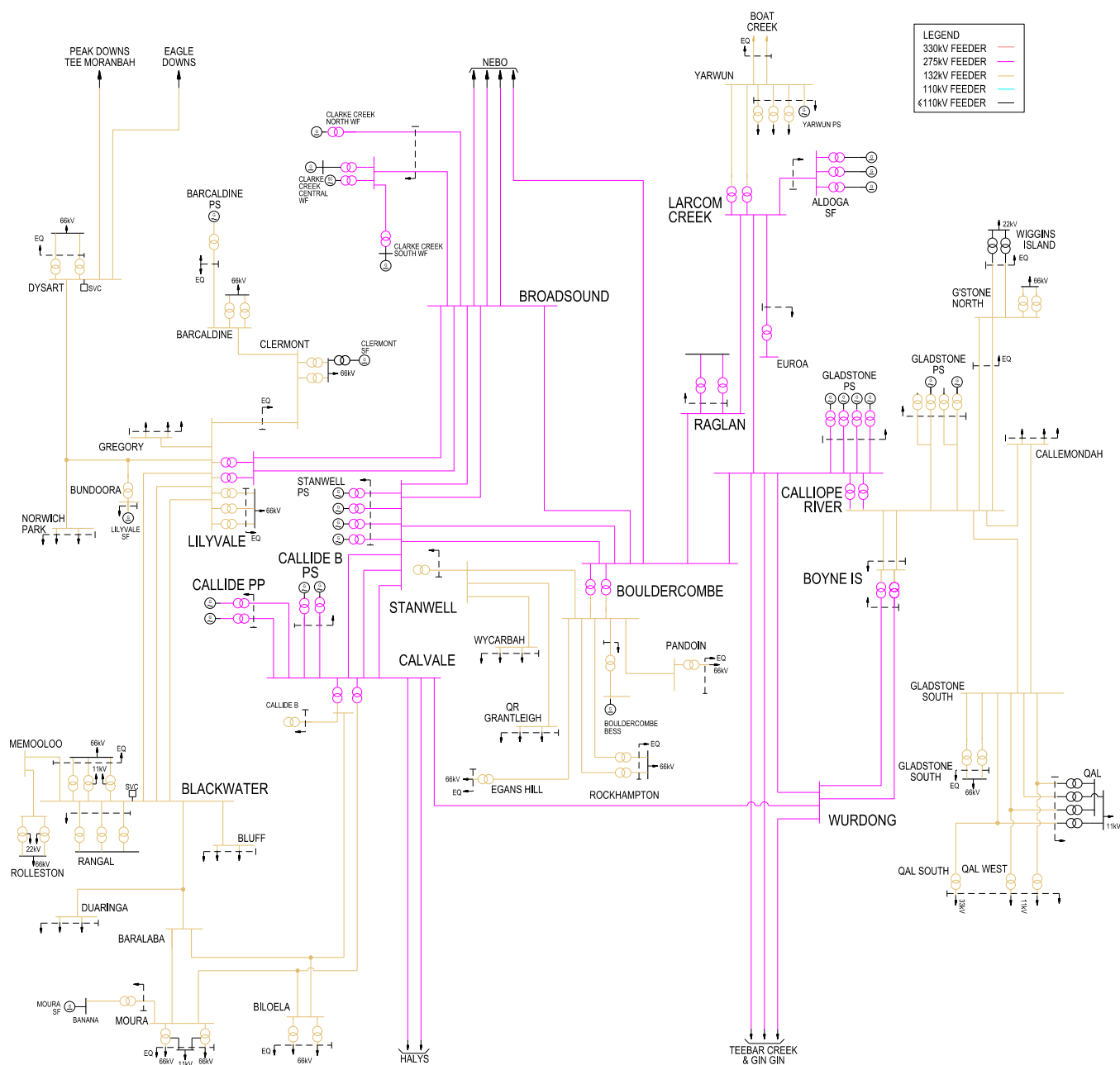
Figure 9.10 Existing high voltage network, July 2026 – Central Queensland
