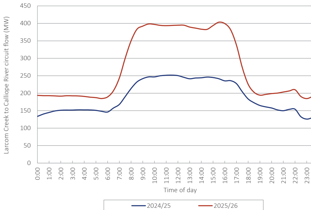
Figure 9.8 Comparison of average daily load on Larcom Creek to Calliope River Circuit
