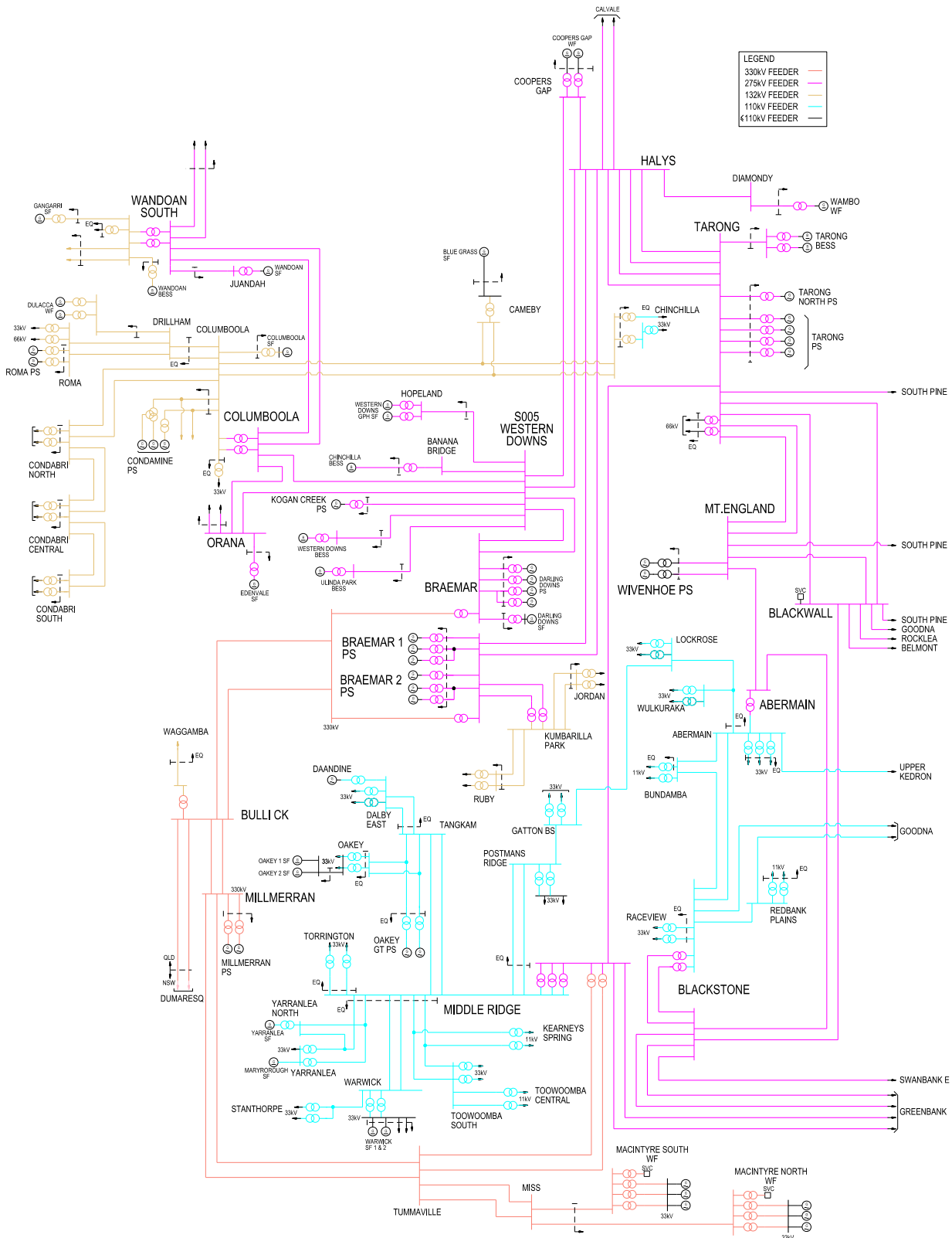
Figure 9.11 Existing high voltage network, July 2026 – South West Queensland
