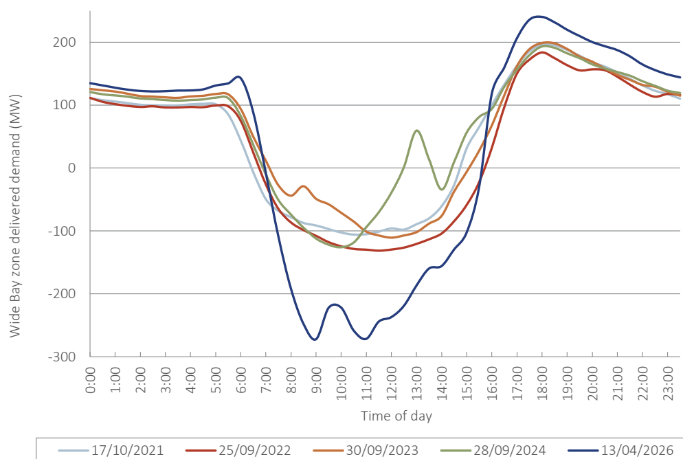
Figure 9.7 Wide Bay daily profile of minimum demand days over the last five years
