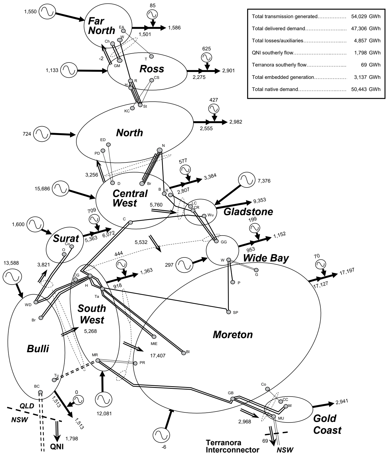
Figure 9.3 Zonal electricity transfers (GWh), 2024/25
