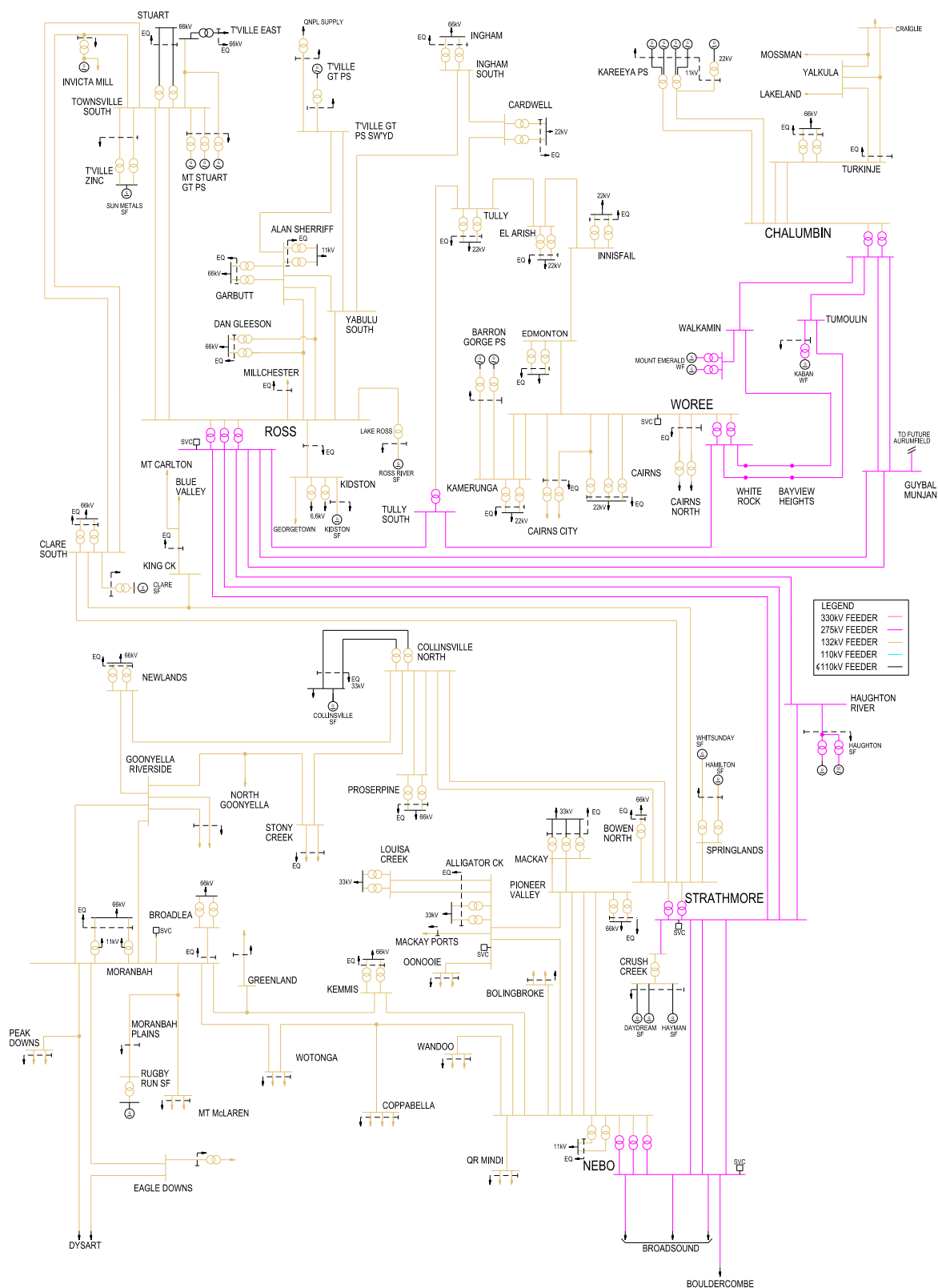
Figure 9.9 Existing high voltage network, July 2026 – North Queensland
