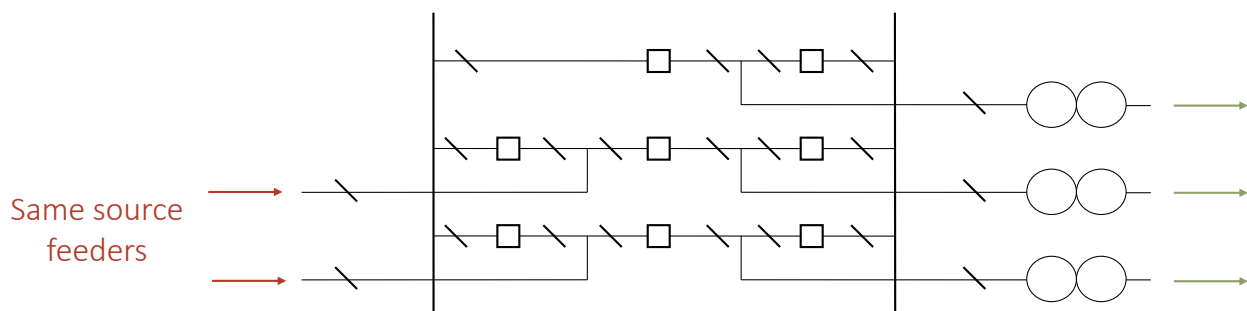
Figure B.1 Typical 1½ CB (Breaker and a Half) bus configuration – radial supply
