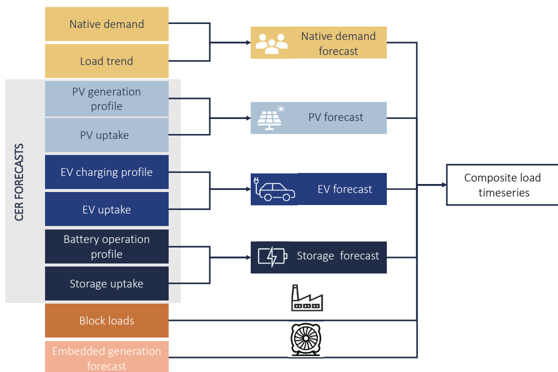
Figure 2.1 Powerlink's forecasting components
