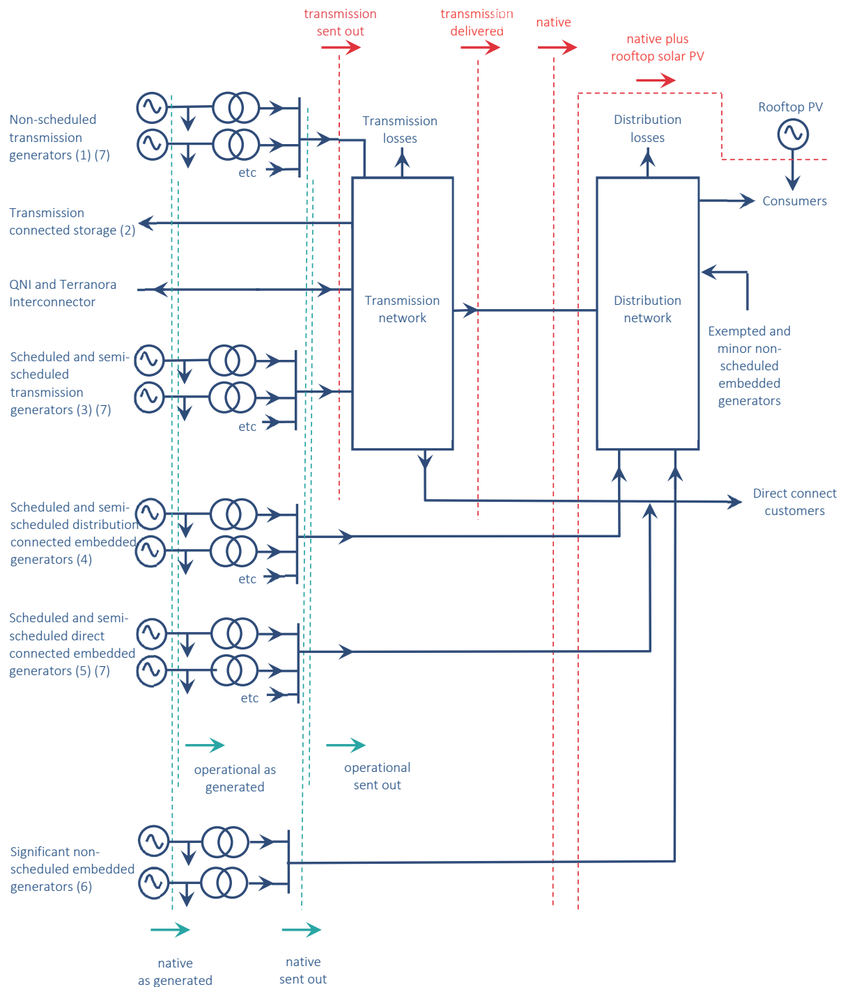
Figure 2.13 Load measurement definitions
