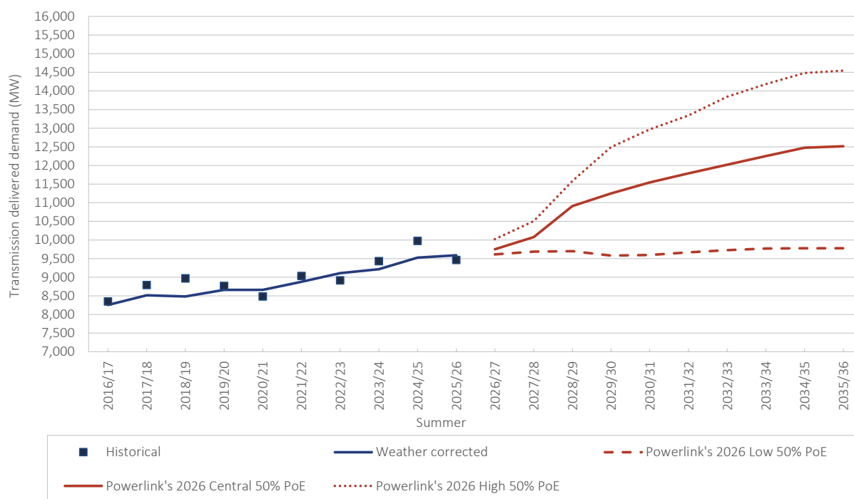
Figure 2.15 Historical and forecast transmission-delivered summer maximum demand
