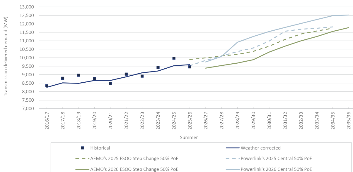
Figure 2.9 Comparison of AEMO's 2025 and 2026 ESOO Step Change scenario forecast with Powerlink's 2025 and 2026 Central scenario 50% PoE transmission-delivered demand forecast
