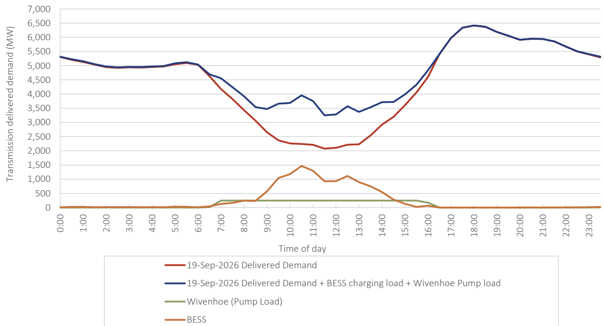
Figure 2.19 Daily load profile of the 2026 annual minimum transmission-delivered demand day and minimum delivered demand plus transmission-connected BESS charging load and Wivenhoe pump load
