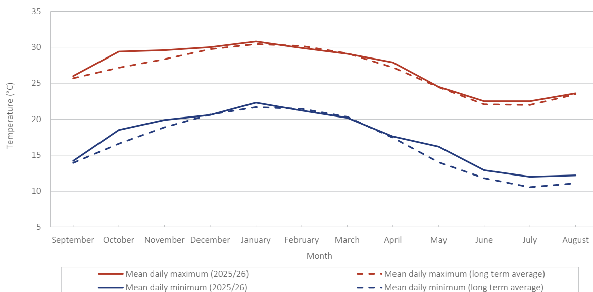
Figure 2.8 Brisbane temperature ranges over September 2025 to August 2026
