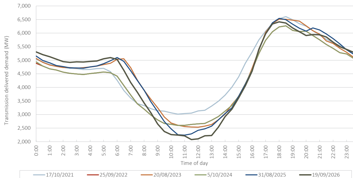
Figure 2.12 Transmission-delivered minimum demand for the Queensland region
