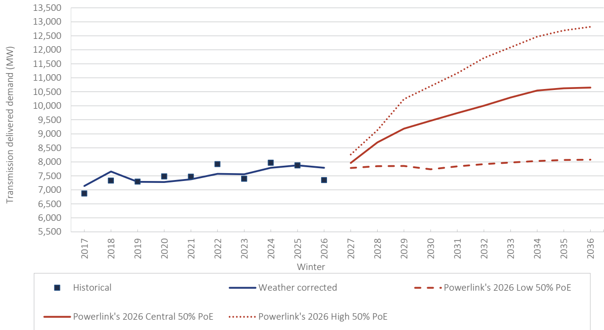
Figure 2.16 Historical and forecast transmission-delivered winter maximum demand
