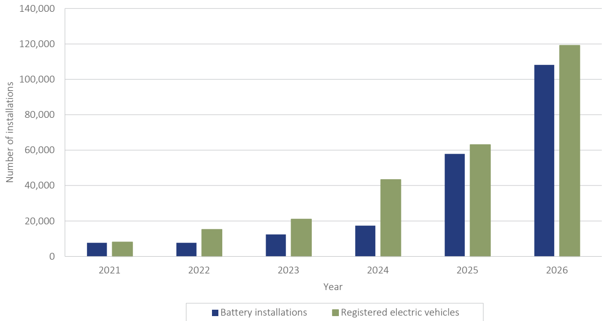
Figure 2.5 Queensland residential battery uptake and number of registered electric vehicles
