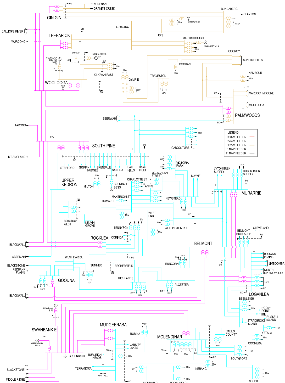
Figure 9.12 Existing high voltage network, July 2026 – South East Queensland
