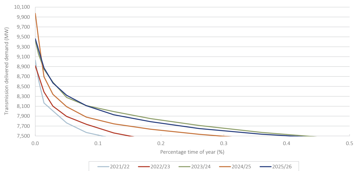
Figure 2.22 Historical transmission-delivered load duration curves (0-0.5%)
