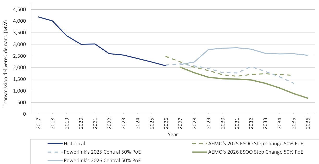
Figure 2.11 Comparison of AEMO's 2025 and 2026 ESOO Step Change scenario minimum delivered demand forecast with Powerlink's 2025 and 2026 Central scenario
