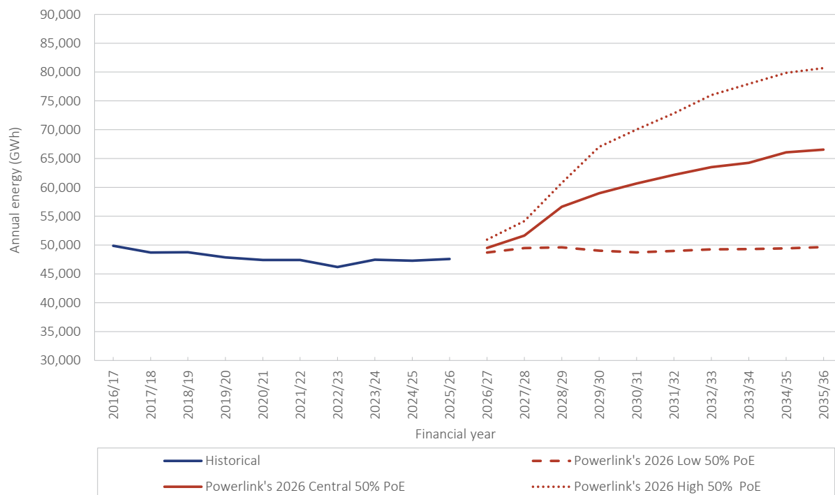
Figure 2.14 Historical and forecast transmission-delivered energy
