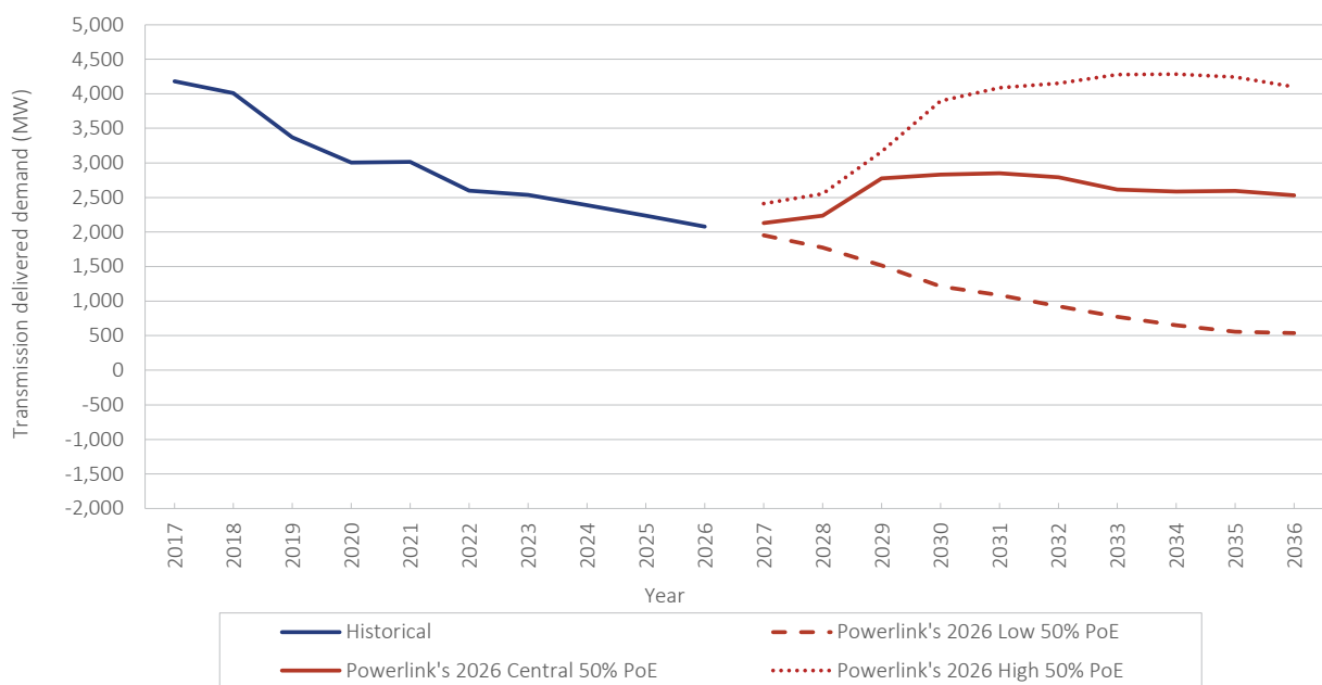
Figure 2.17 Historical and forecast transmission-delivered annual minimum demand
