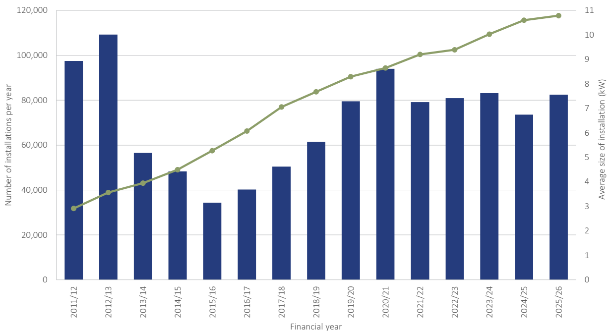
Figure 2.3 Annual installation rates and average sizes for Queensland rooftop solar PV panel capacity
